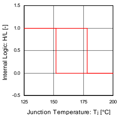
Fig.10 Thermal shutdown
