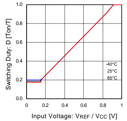
Fig.6 VREF - DUTY (VCC=12V)
