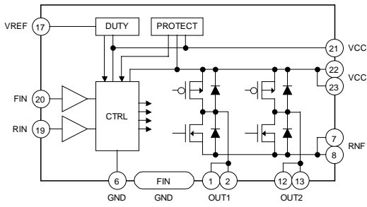
Fig.29 BD6222FP
